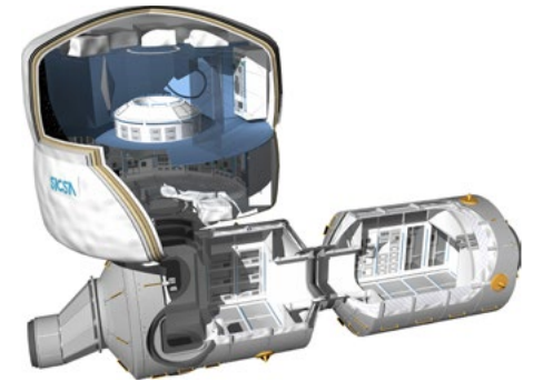
Transhabitat for Mission to Mars Image credit: SICSA, Boeing, ILC Dover for NASA, 2008-2009 SICSA, University Houston
