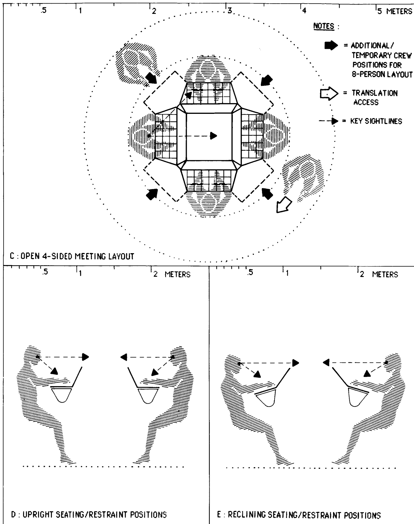
FIGURE 16 - GROUP MEETINGS : VOLUMETRIC ENVELOPES
