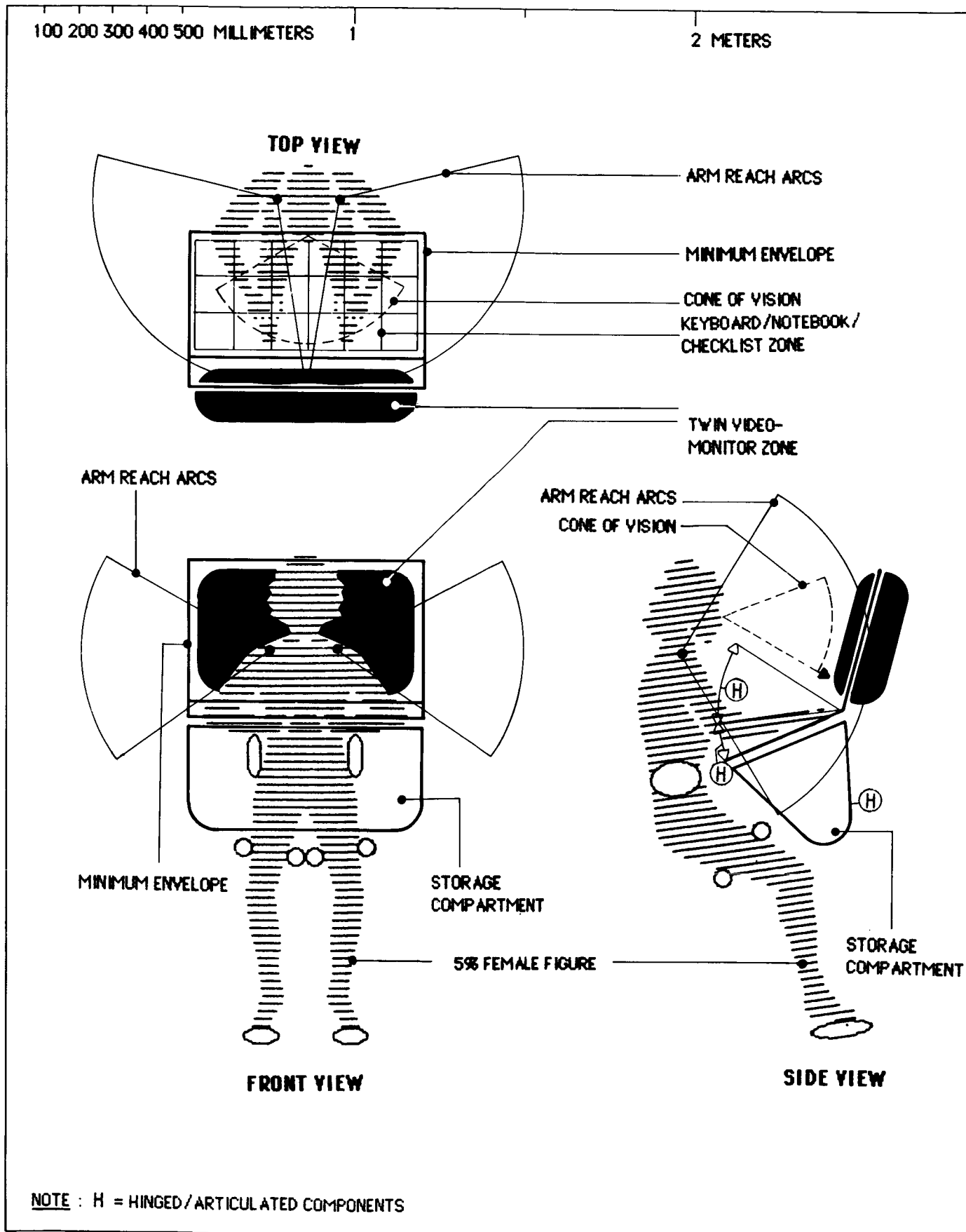
FIGURE 12 - PLANNING AND TRAINING : MINIMUM ERGONOMIC ENVELOPE
